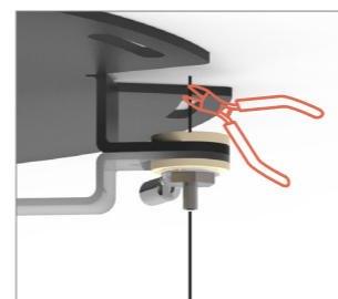
8. Cut the excess of wire. Wires can not be in contact with conductive surfaces, dont leave more than 1cm
